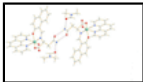
Fig. 2. Hydrogen bonding interactions in the title compound shown as dashed lines.
